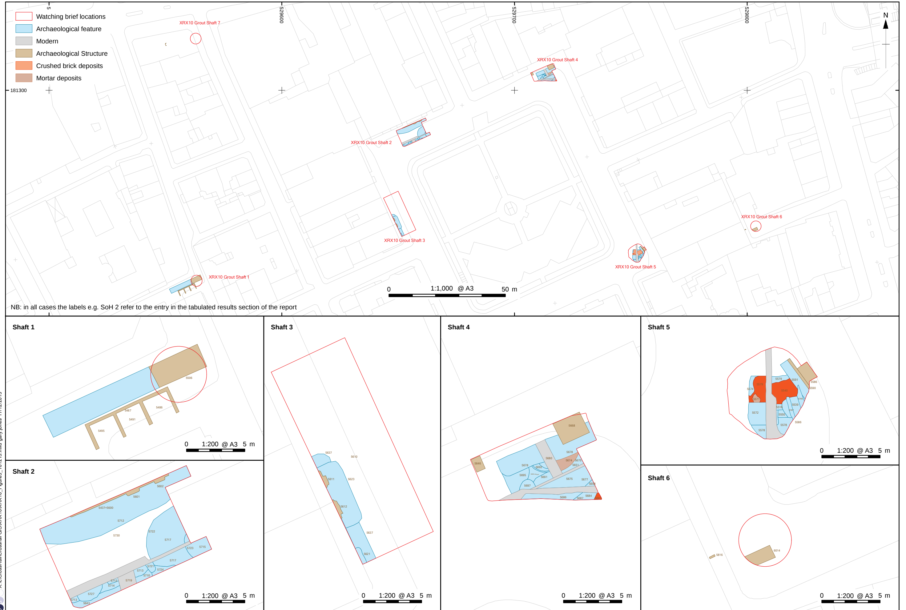
Figure 3: Location of Grout shaft Works around the Tottenham Court Road Station (Western Ticket Hall)
